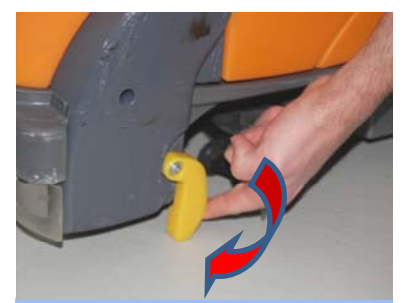
20. Bring machine into parking position by lifting machine a bit with its handle, and flipping the parking lever manually
